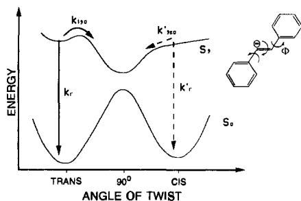
Figure 1. A schematic representation of the isomerization coordinate is shown for reaction from both the trans and cis sides. The rate constants k_{120} and k'_{120} are for isomerization on the singlet surface and the rate constants k_r and k'_r are for radiation.
