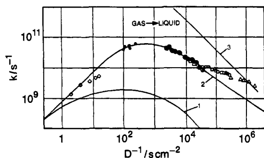
Figure 18. Isomerization rates of trans -stilbene are plotted versus the inverse of the diffusion constant in alkane solvents [gaseous methane ( \diamond ), gaseous ethane ( \bullet ), liquid ethane ( \circ ), liquid alkanes ( \square ), and compressed hexane ( \Delta )]. Curve 1 is the prediction of "standard" RRKM theory and curve 2 is the same model with a modified barrier. Curve 3 represents the rates for isomerization in alcohol solvents. Reproduced from ref 106b. Copyright 1986 American Chemical Society.
